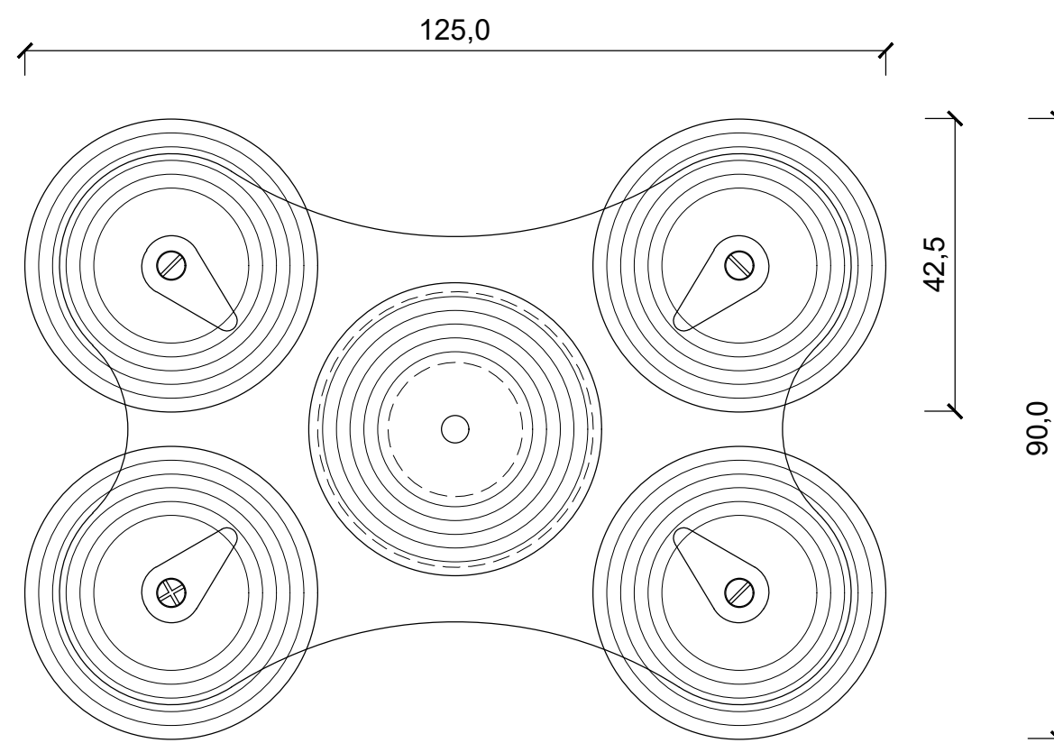
Plan View
