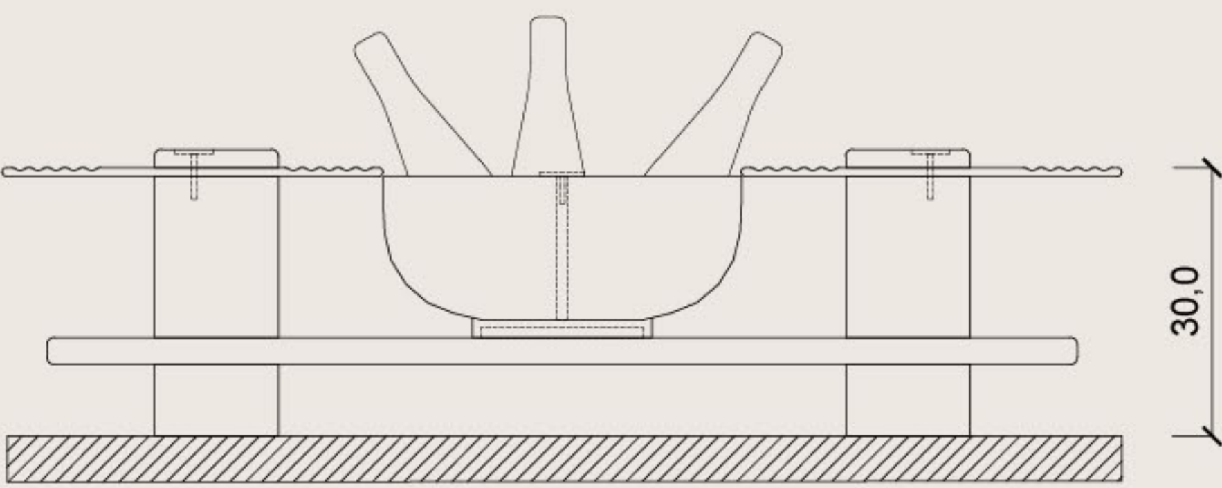
Side View
