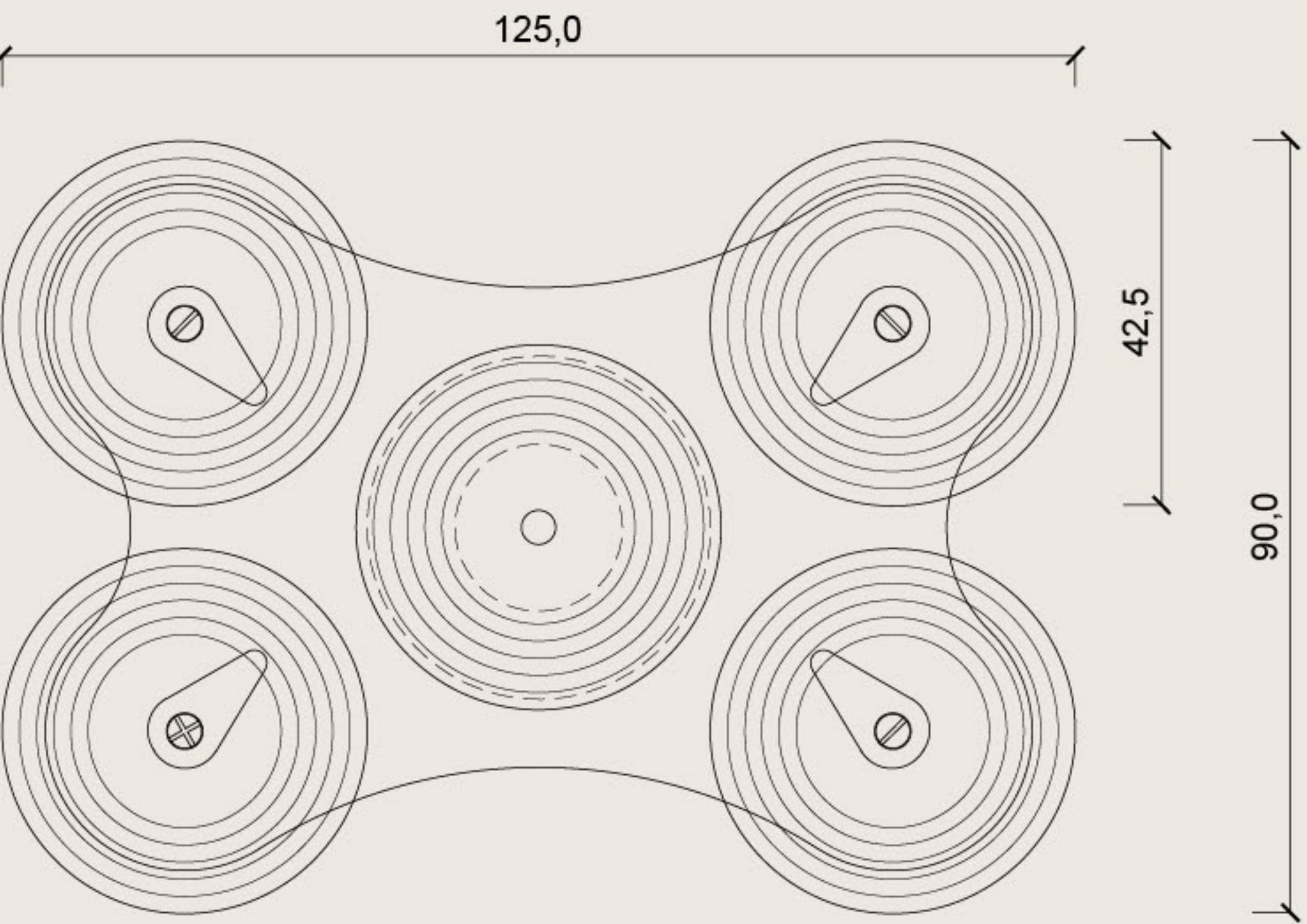
Plan View
